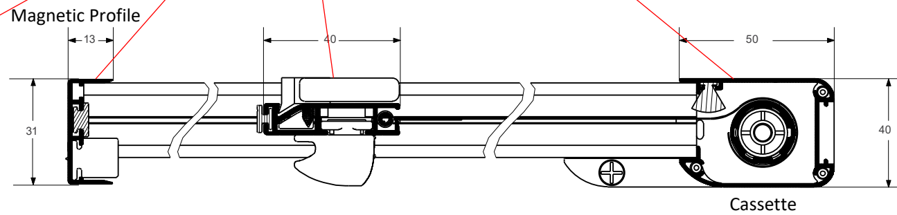
Horizontal Section
