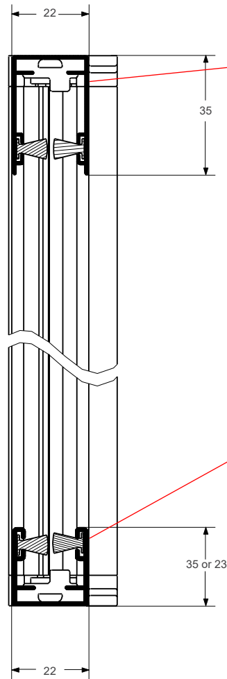
Vertical Section
