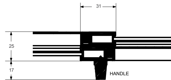
TOP VIEW SHOWING OVERLAPPING FRAMES
